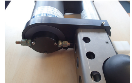
SeaFET connected to MicroCAT pumped flow path
