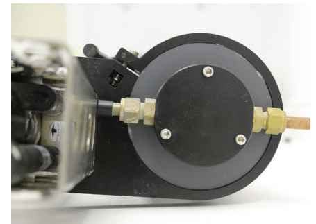
SeaFET connected to MicroCAT pumped flow path
